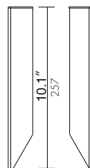
LWP0100 PEG FOR GROUND FIXING
